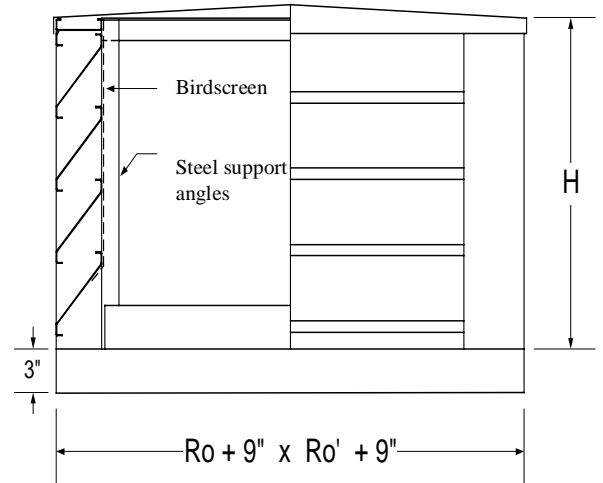
45 Degree Plain Blade Shown (Model MFL-24)
